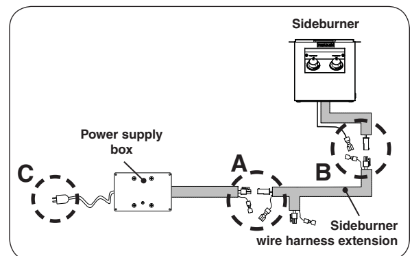
Fig. 13-4 Connect sideburner to power supply
