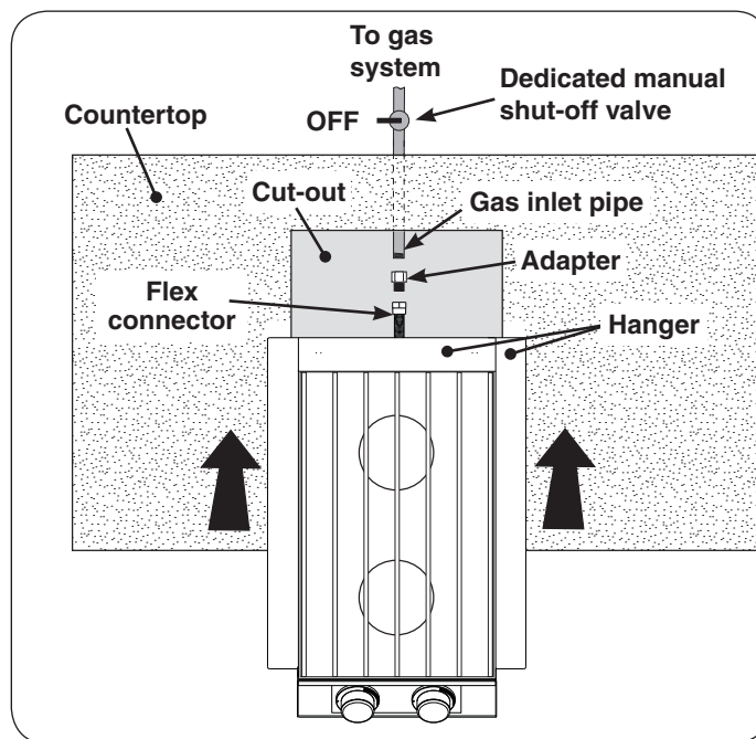
Fig. 12-3 Gas connection diagram
