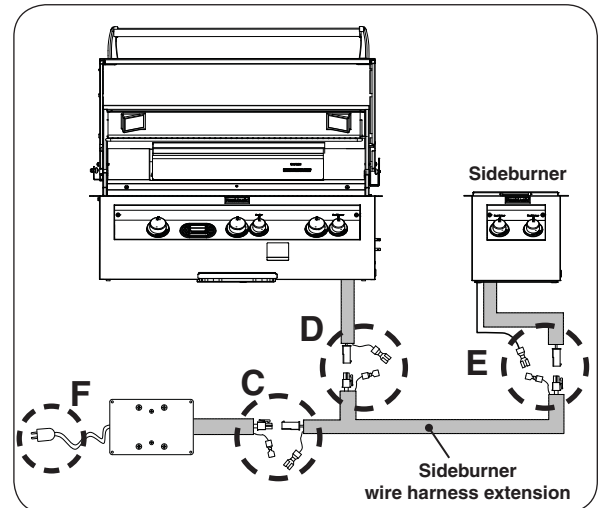
Fig. 13-3 Connect sideburner to grill setup
