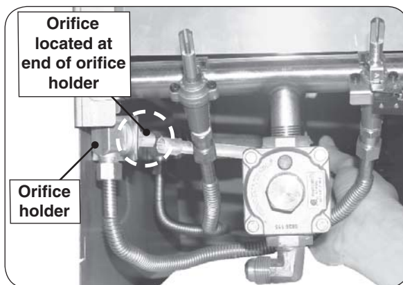
Fig. 16-3 Orifice location
